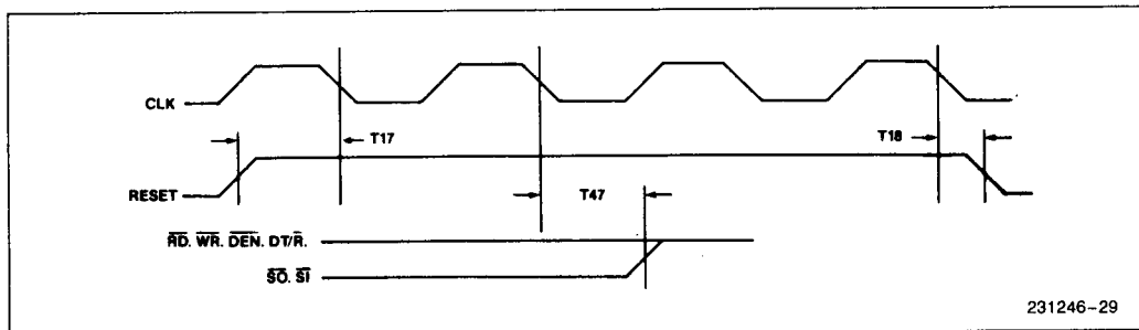
Figure 28. RESET Timing
