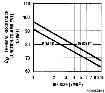
FIGURE 8. Thermal Resistance vs Board or Socket Mount
