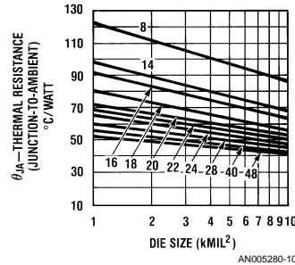
FIGURE 10. Thermal Resistance vs Die Size vs Package Type (Molded Package)
