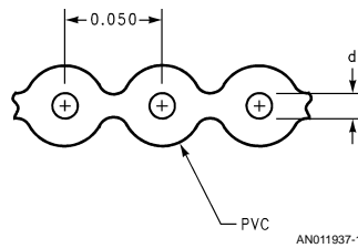
FIGURE 1. Drawing of Flat Cable, Cross-Section
