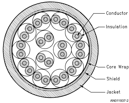
FIGURE 2. Drawing of Round Cable, Cross-Section
