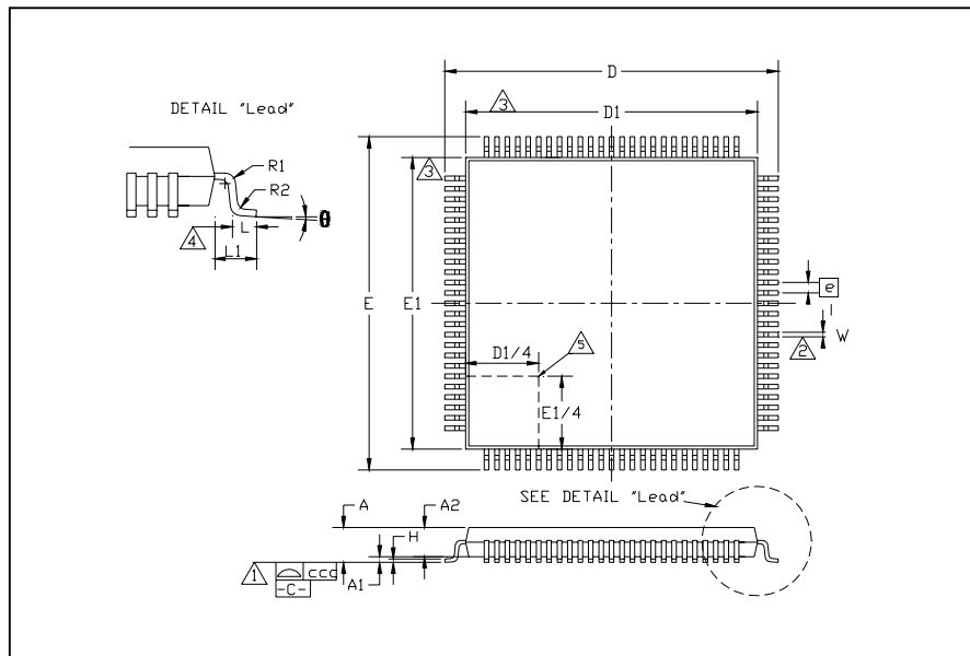
Figure 9.1 - 100 Pin TQFP Package Outline, 12x12x1.4 Body, 2MM Footprint (Rev A)
