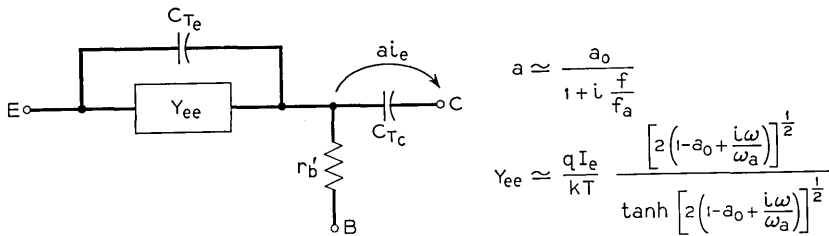
Fig. 5 — Equivalent circuit of the p-n-i-p transistor.
