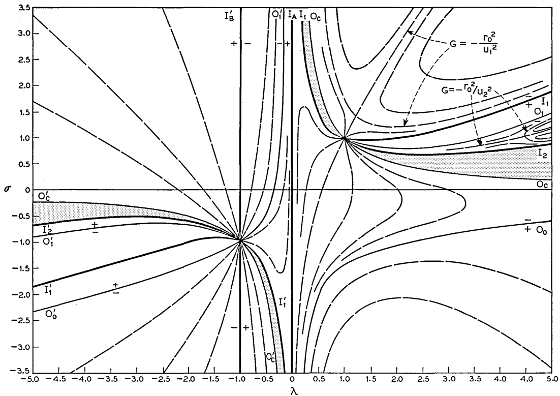
Fig. 5 — Contours of constant G(\lambda, \sigma) for r_0 = 2.2 . Scales distorted to show saddle points. G assumes any given value infinitely often in the shaded regions.
