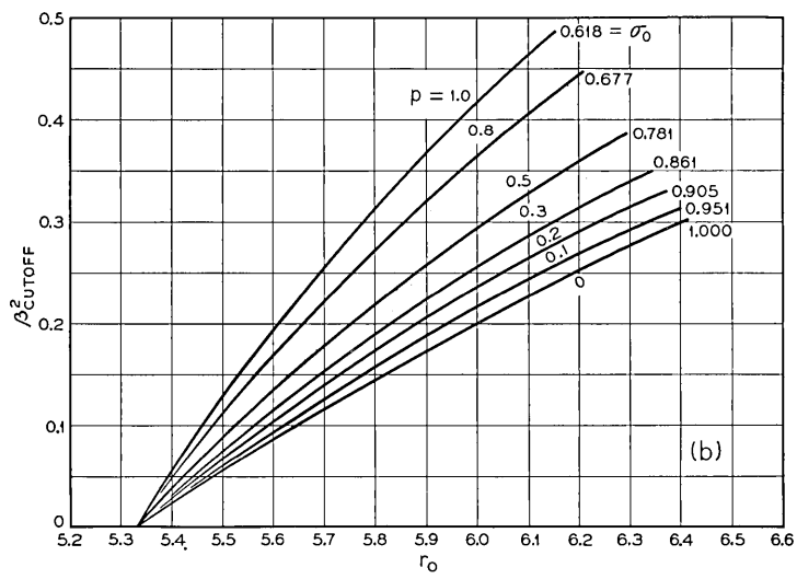
Fig. 11 — \beta^2 at the type 2' cutoff as a function of r_0 for various p . 2 0 ' cutoff, TE 11 -limit mode; (b), 2 1 ' cutoff, TM 11 -limit mode. The presence of a curve for p = 0 is clarified in the text.
