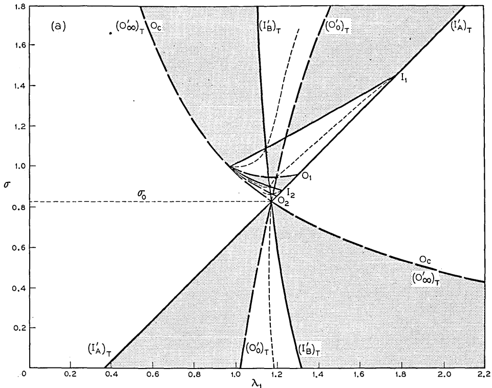
Fig. 9 — Geometrical exploration of the solution curves. The permitted areas of the \lambda - \sigma plane are divided by the O, I, (O)_T, (I)_T curves into regions in which G(\lambda, \sigma) and G(T(\lambda), \sigma) have like or unlike signs. Shaded regions are those of unlike signs. Solution curves (shown schematically by dotted lines) must lie in regions of like signs. Only the first few O and I curves are shown. Fig. 9(a) and (b), r_0 \sim 3.0 ; Fig. 9(c) and (d), r_0 \sim 5.0 ; Fig. 9(e) and (f), u_2 < r_0 < j_2 ; Fig. 9(g), r_0 < u_1 . |p| < 1 , throughout. The horizontal dashed line marks |\sigma| = |\sigma_0| .
