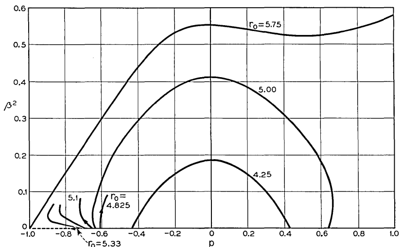
Fig. 10(b) — \beta^2 versus \rho for small values of \sigma — the TM_{11} -limit mode.
