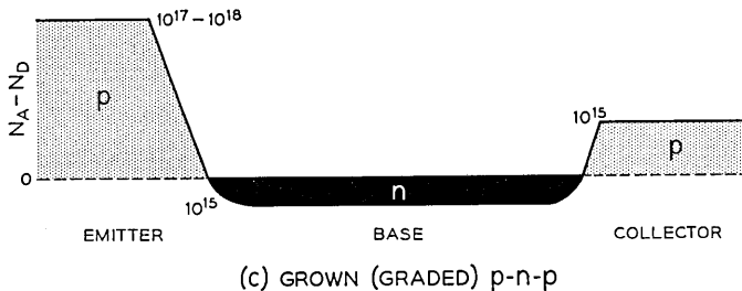
Fig. 2 — Impurity density profiles.
