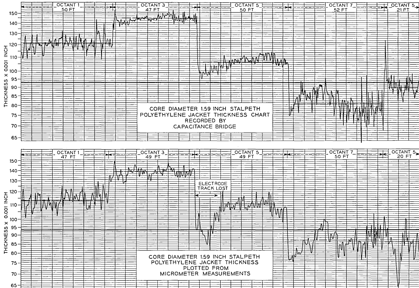
Fig. 12 — Accuracy check under operating conditions.
