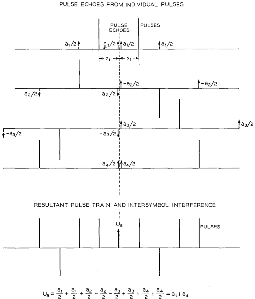
Fig. 31 — Combination of pulse echoes into intersymbol interference for a particular case.
