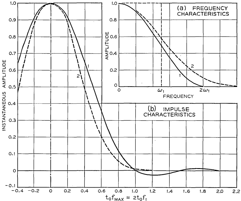
Fig. 18 — Comparison of two representative frequency and impulse transmission characteristics. Frequency characteristic 1: T(\omega) = \frac{1}{2}[1 + \cos \pi\omega/2\omega_1] . Frequency characteristic 2: T(\omega) = \exp - 0.54(\omega/\omega_1)^2 .
