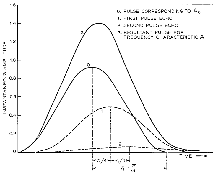
Fig. 28 — Modification of impulses characteristic by slow cosine variation in amplitude characteristic.
