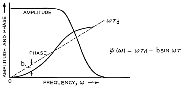
(a) LOW-PASS CHARACTERISTIC
