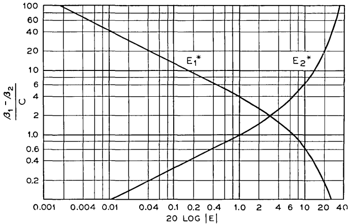
Fig. 18 — Wave amplitude factors at the maximum power transfer value of \underline{cx} versus (\beta_1 - \beta_2)/c when the coupled lines have equal attenuation constants.
