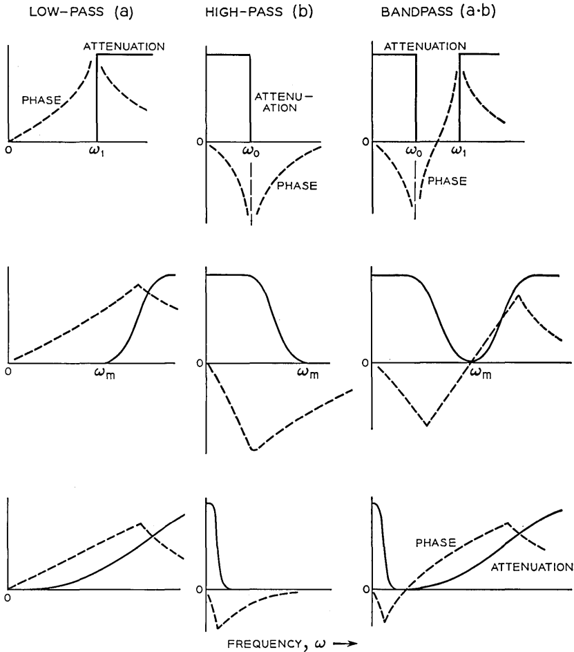
Fig. 4 — Attenuation and phase shift for various types of transmission frequency characteristics.
