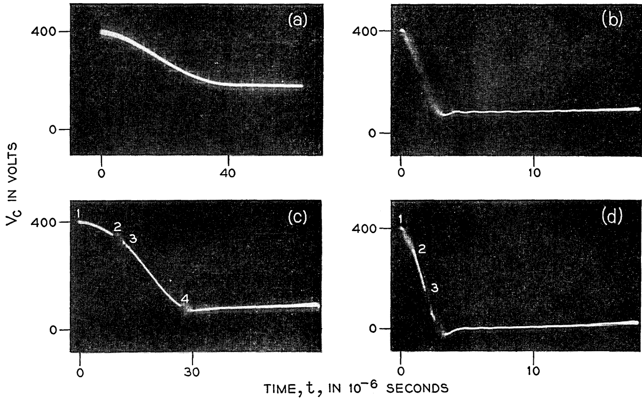
Fig. 14 — Voltage transients at circuit condenser. A: all glow. B: no glow, only a series of interrupted arcs. C: glow-interrupted arcs — steady arc. D: no glow, interrupted arcs — steady arc — interrupted arcs.
