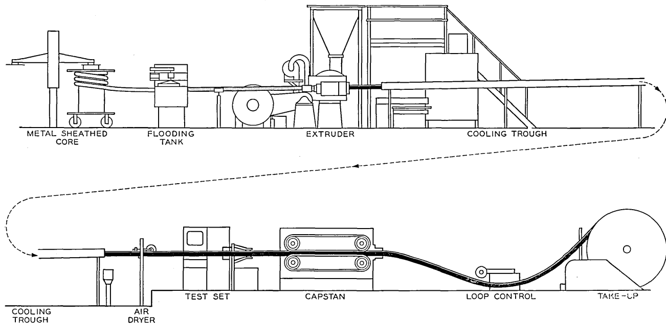
Fig. 13 — Polyethylene sheathing line.
