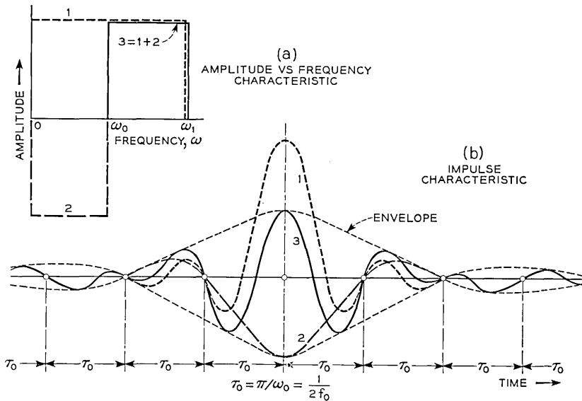
Fig. 9 — Special case of idealized band-pass characteristic in which \omega_1 = 2\omega_0 and resultant impulse characteristic is zero at intervals \tau_0 = \frac{1}{2f_0} .
