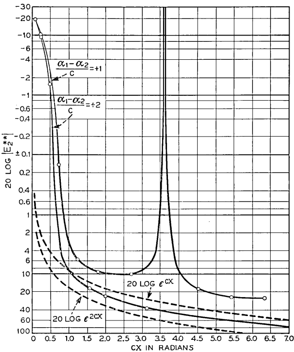
Fig. 28 — Undriven line wave amplitude versus cx , for equal phase constants; (\alpha_1 - \alpha_2)/c as a parameter.
