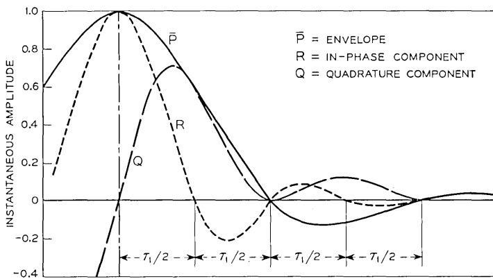
(b) IMPULSE CHARACTERISTIC
