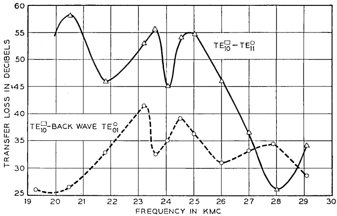
Fig. 48 — Circular electric wave directivity and one unwanted mode (TE 11 ○ ) output versus frequency for the transducer of Fig. 42.
