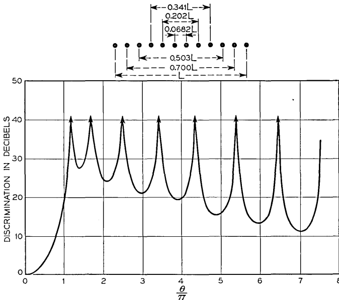
Fig. 13 — Discrimination for 12 equal-strength point couplings arranged to simulate the continuous distribution of Fig. 4, line 2.
