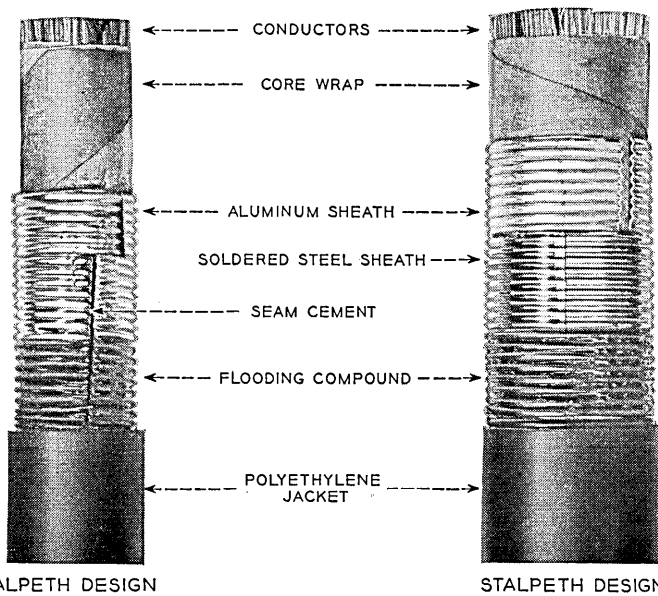
Fig. 1 — (Left) Telephone exchange cable of Alpth design; (right) Stalpth design.
