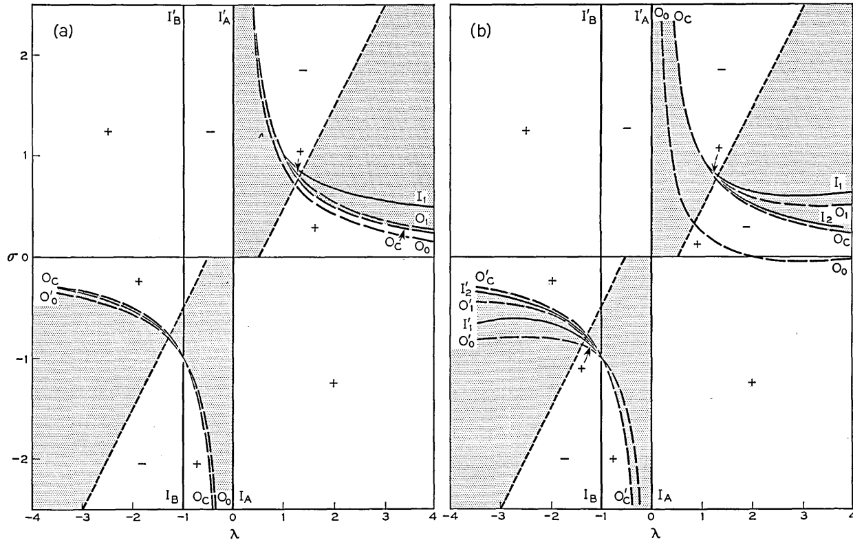
Fig. 8 — The division of the parts of the \lambda - \sigma plane allowed by the Polder relation, Equation (31b), into regions of positive and negative G by the first few O and I curves. Excluded regions are shaded. |p| is about 0.5. Fig. 8(a), 0 < r_0 < 1 ; Fig. 8(b), 1 < r_0 < u_1 ; Fig. 8(c), r_0 = u_1 ; Fig. 8(d), u_1 < r_0 < j_1 ; Fig. 8(e), j_1 < r_0 < u_2 .
