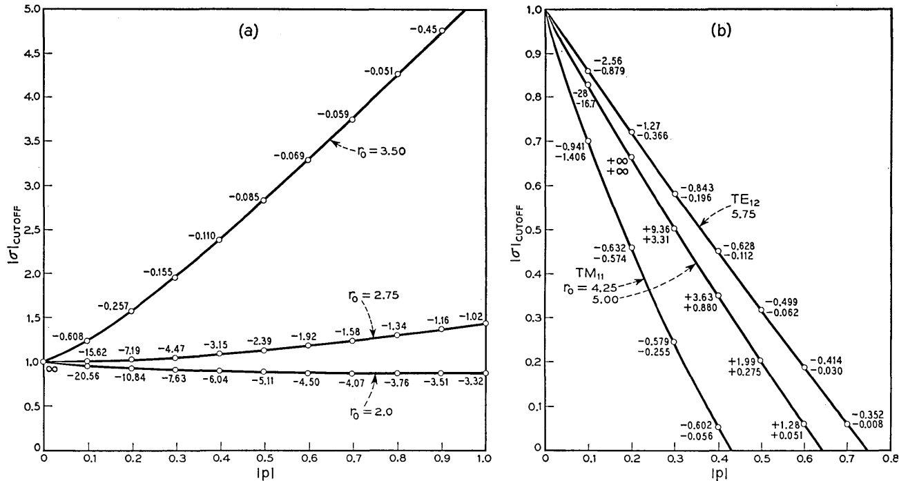
Fig. 12 — Type 1 cutoff. |\sigma| versus |p| for some values of r_0 . (a) refers to the \text{TM}_{11} -limit mode in its incipient stage; the number attached to the points are values of \frac{d\beta^2}{d\sigma} \text{sgn } p at the cutoff. (b) refers to the fully developed \text{TM}_{11} -limit and \text{TE}_{12} -limit modes in the region |\sigma| < |\sigma_0| : the upper attached number is \frac{d\beta^2}{d\sigma} \text{sgn } p and the lower attached number \frac{d\beta^2}{dp} \text{sgn } p .
