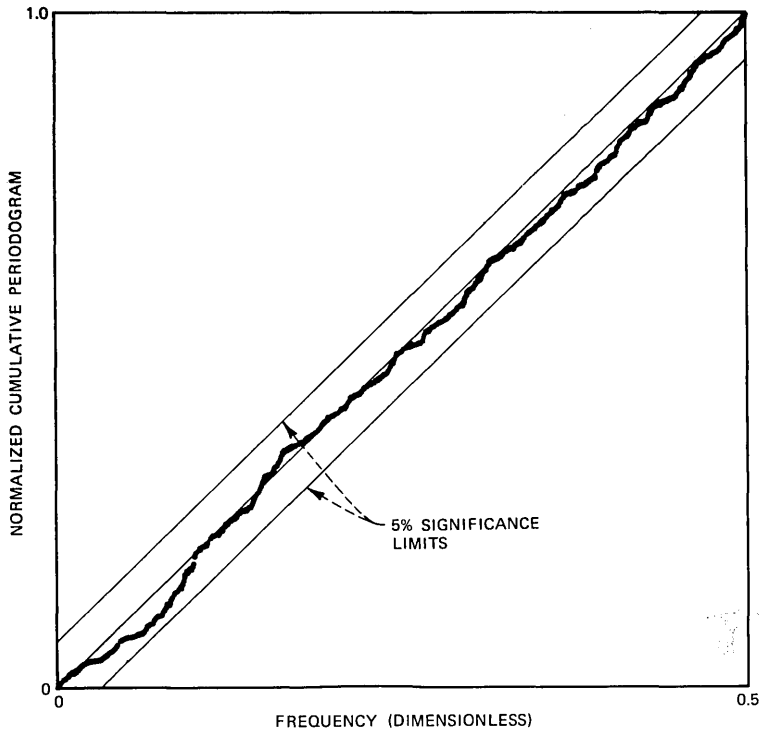
Fig. 31—Normalized cumulative periodogram for line 1 time intervals between bursts, T_{upper} = T_{lower} = 800 ( N = 768 ).
