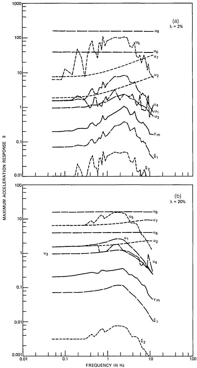
Fig. 3—Response bounds of single-degree-of-freedom structures subjected to random load.
