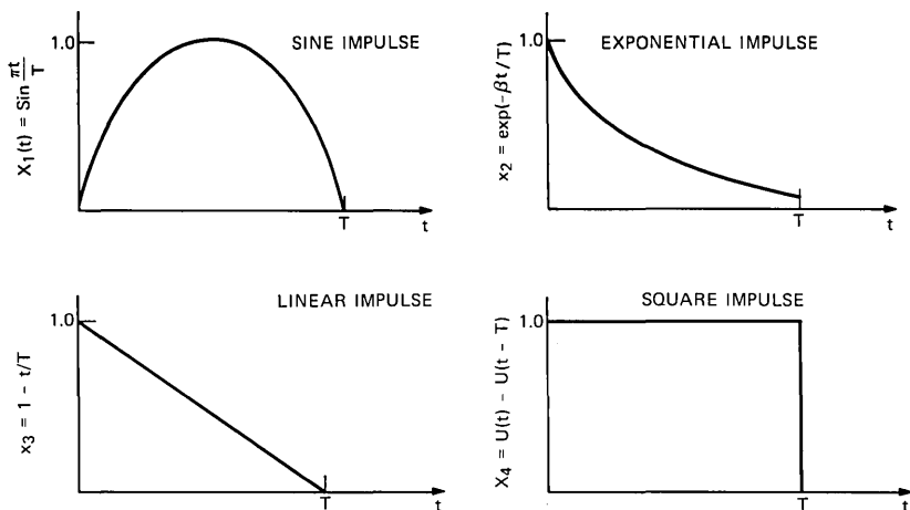
Fig. 2—Impulse loads.
