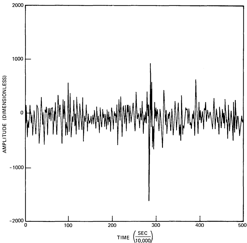
Fig. 4—Typical line 1 telephone noise waveform (filtered).
