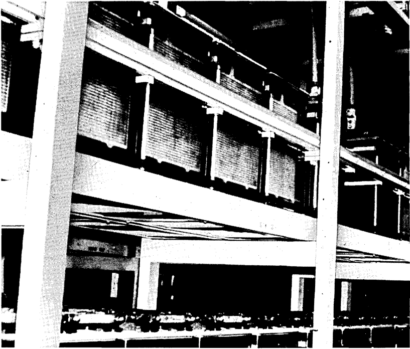
Fig. 5—Soft-site battery stand modified for service in earthquake area.
