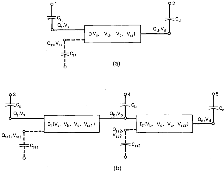
Fig. 2—Lumped-charge model including the effect of interface states for the transfer of charge through a single stage of a CTD. (a) Single-step transfer. (b) Two-step transfer.
