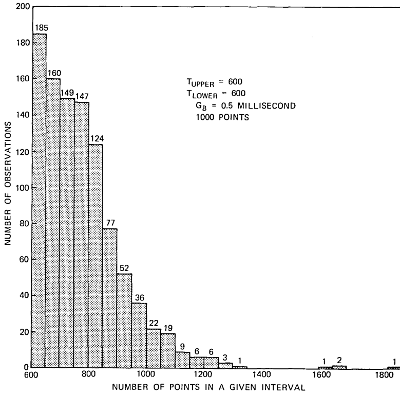
Fig. 35—Histogram of maximum burst amplitudes ( N = 1000 ).
