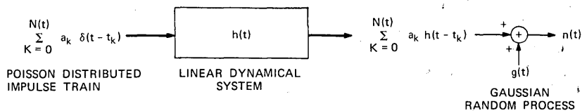
Fig. 24—Block diagram for generating a gaussian-plus-filtered-Poisson process.
