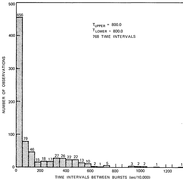
Fig. 27—Histogram for line 1 time intervals between bursts ( N = 768 ).
