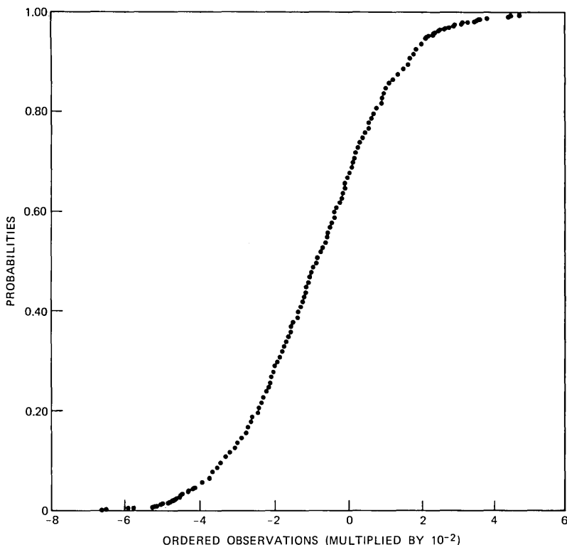
Fig. 10—Typical line 1 empirical cumulative distribution function ( N = 1000 ).
