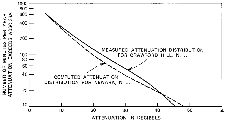
Fig. 14—Comparison of measured attenuation distributions at Crawford Hill, N. J., with computed attenuation distributions from rain rate data from Newark, N. J. for three years (1967 to 1969), vertical polarization.
