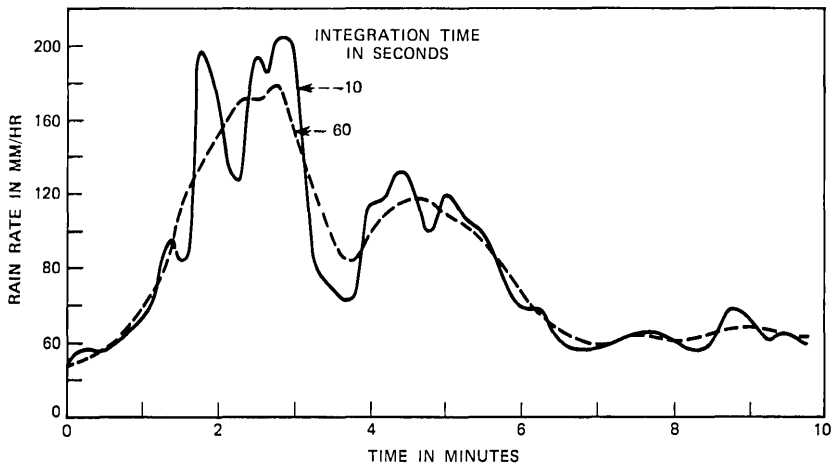
Fig. 4—Integrating rain gauge: storm of April 3, 1972.
