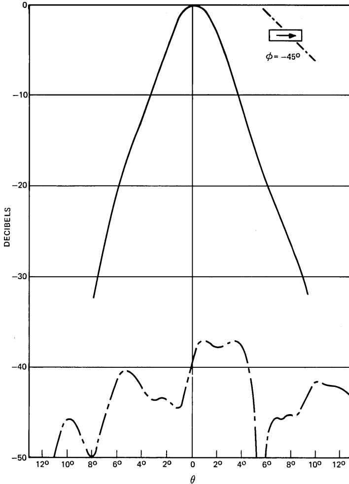
Fig. 12—Radiation patterns of horizontally polarized double-cylinder antenna measured at 18.5 GHz in the \phi = -45^\circ plane for the main component (—) and the cross-polarized component (---) of the far field.
