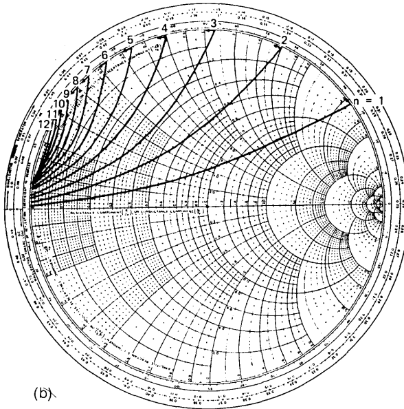
Fig. 10—Normalized stability charts for external impedance. (Arrows indicate stable regions. Z_0 C \pi / \tau_d = 1.25 \text{ ohm } F S^{-1} .) (a) \bar{x}_d = 0.83 , \omega_a \tau_d = 0.4\pi . (b) \bar{x}_d = 0.83 , \omega_a \tau_d = 0.8\pi .
