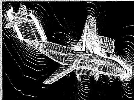
Asuka plane simulation based on Euler equations.
