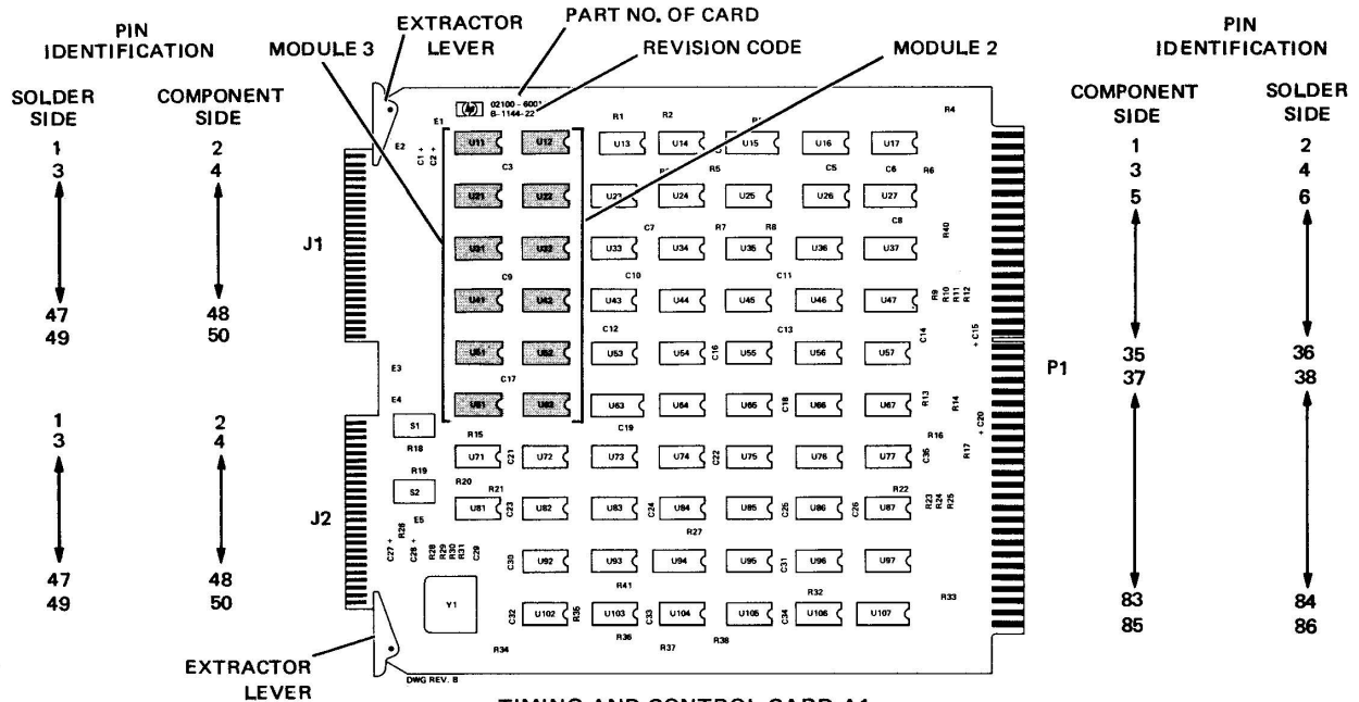
VIEW C
