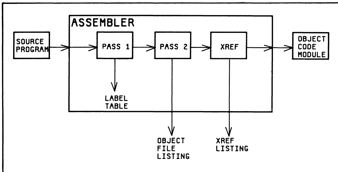
Figure 6-1. Assembly Flow Diagram
