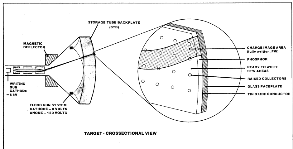
Figure 1. Operation of the direct view storage tube. Flood electrons continuously bombard the phosphor. In the absence of writing-gun electrons, flood electrons maintain the phosphor at the flood-gun cathode potential of 0 volts. When writing-gun electrons strike the phosphor, the phosphor is charged past a threshold to maintain a stored charge image.
