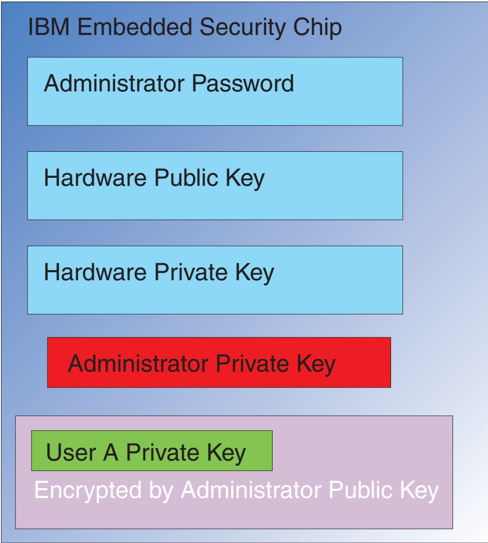
Figure 6. User A's private key, which is encrypted by the Administrator public key, is passed into the security chip.
