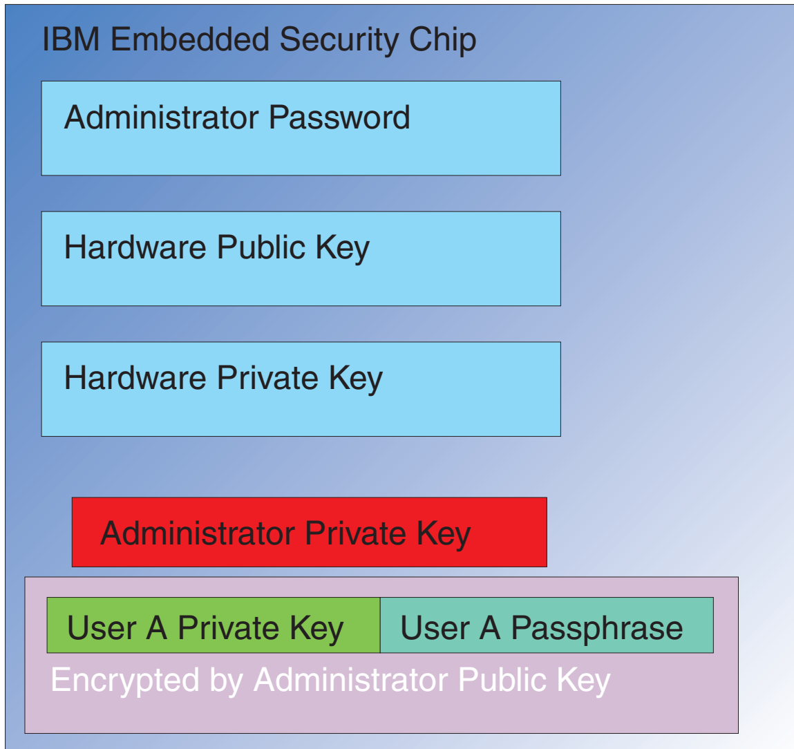
Figure 18. The Administrator's private key is decrypted in the chip.
