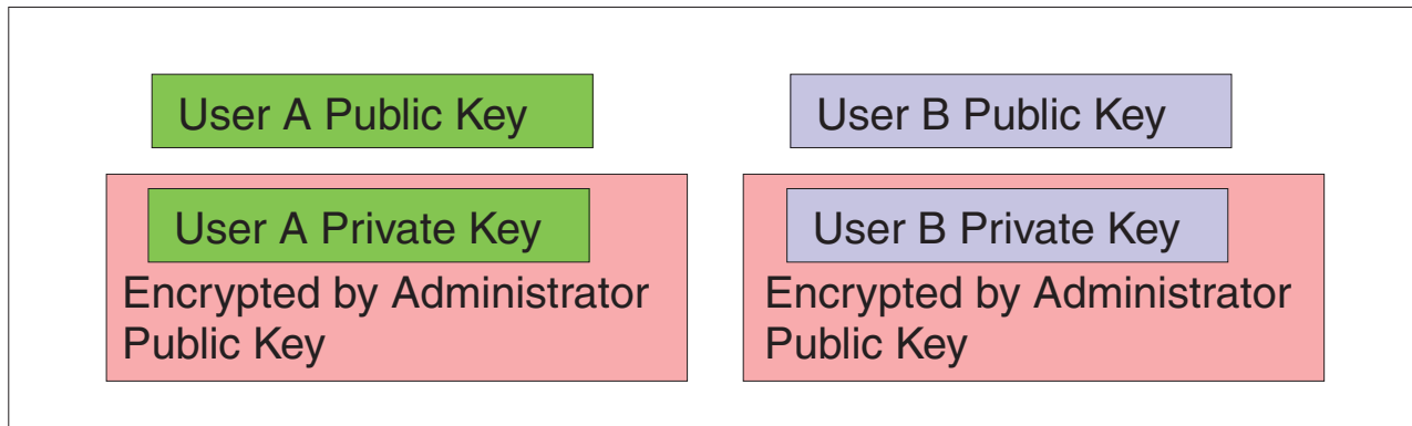
Figure 8. The user-specific private key information is encrypted with the Administrator public key.
