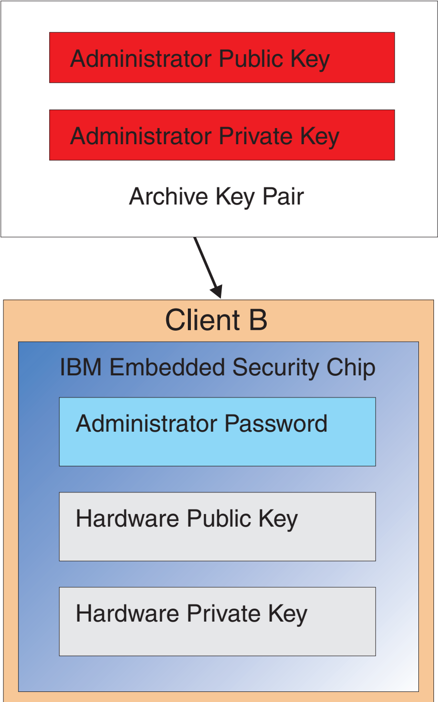
Figure 12. Client B retrieves the Administrator public and private keys from the archive location.
