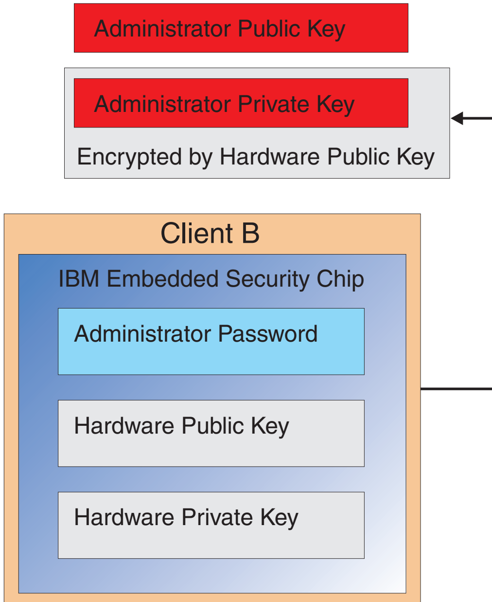
Figure 13. The Administrator private key is encrypted with the Client B hardware key.
