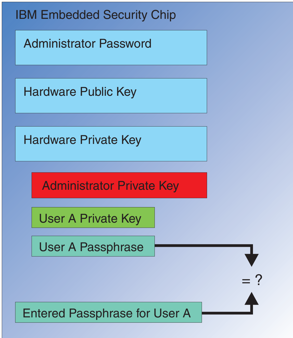
Figure 20. When User A attempts to use the credentials of User A then a passphrase dialog will open.
