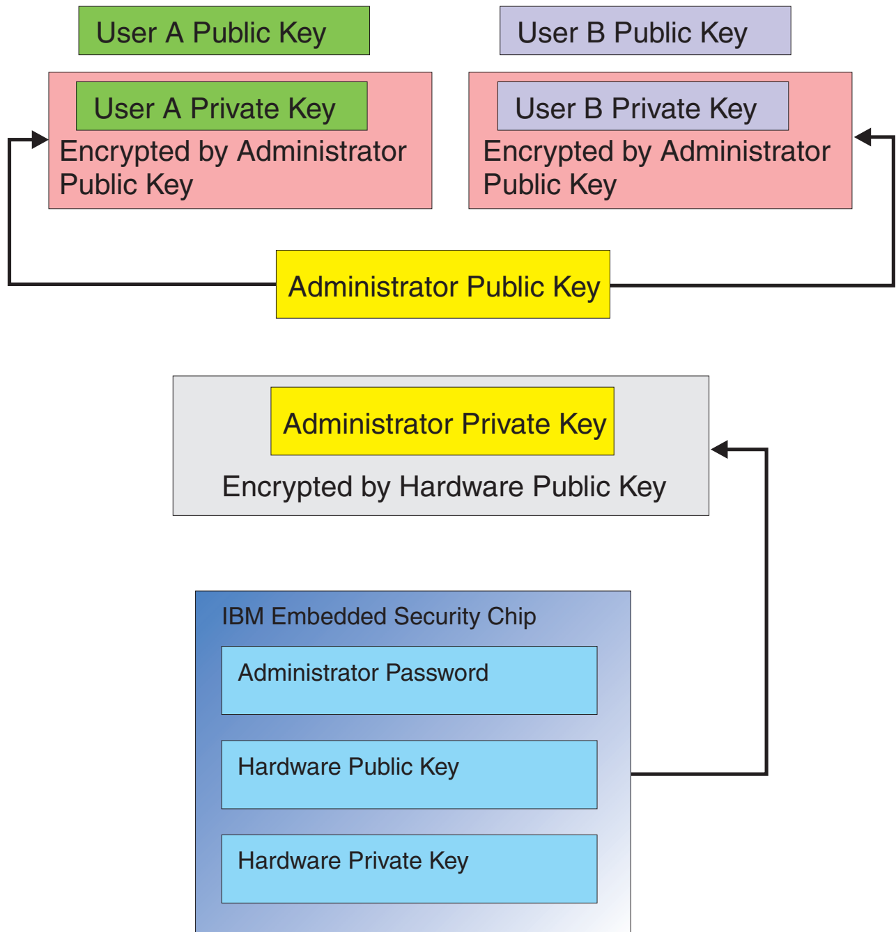
Figure 3. Several layers of encryption provide strong security
