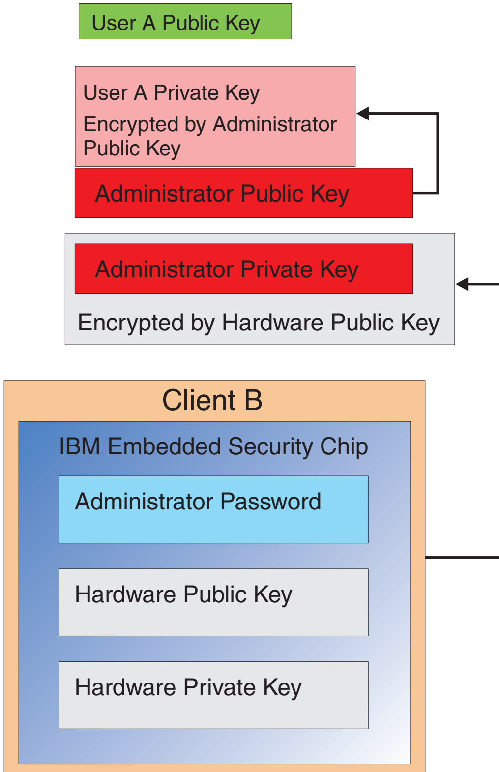
Figure 15. User A is fully restored on Client B.
