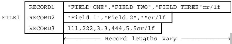
Figure 5-1 Sequential File
