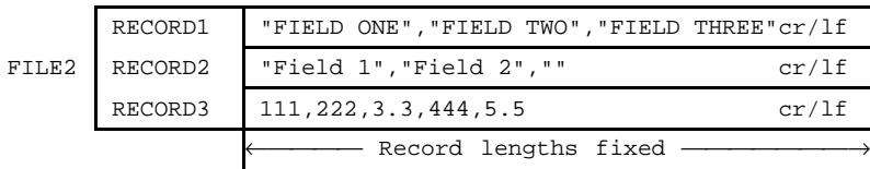
Figure 5-2 Relative File
